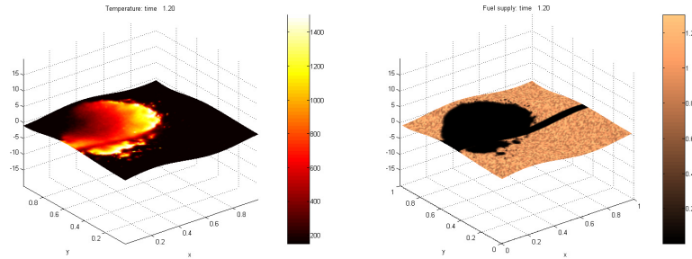
Figure 3. Wind driven wildfire jumping a fire line, modeled by the stochastic reaction-convection-diffusion equation with spotting (1)-(3). Left: fire temperature, Right: fuel supply.
